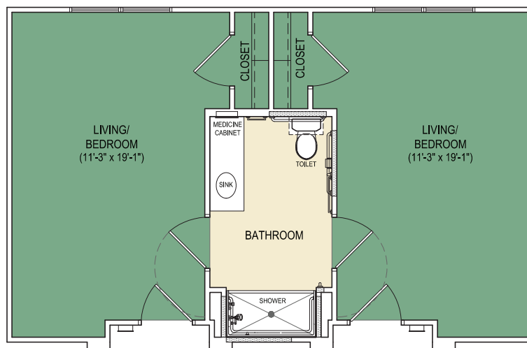
G Studio Semi-private 600 Sq. Ft.
